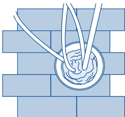
Step 6: Start applying mortar (min. 25-50 mm) on the prepared surface.
